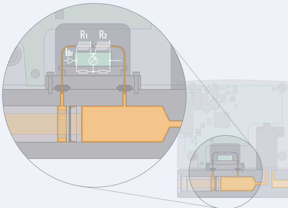
Functional schematic of the capillary sensor
