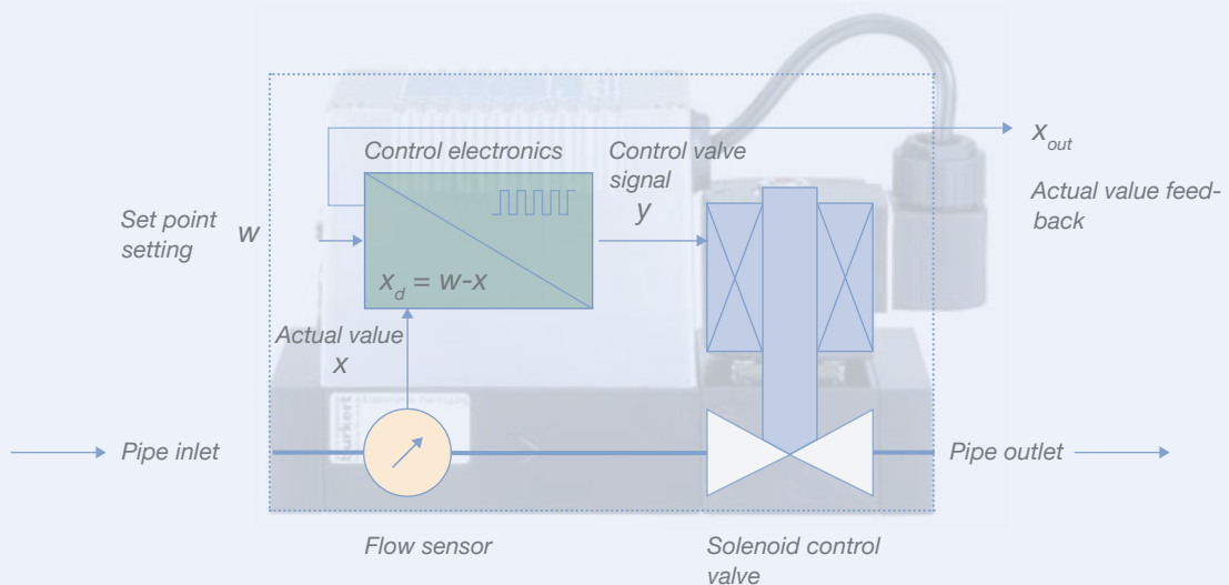
Basic principle closed control loop
