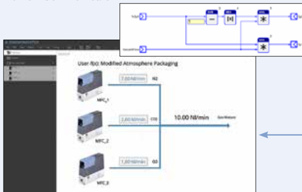
Bürkert Communicator
