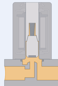
Opened state
