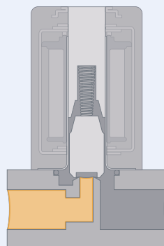
Closed state
